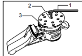
1. Hex wrench 2. Screw 3. Pad
