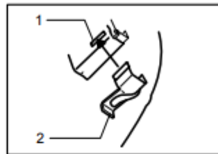
1. Hole 2. Carbon brush cap
