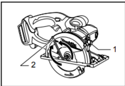
1. Shaft lock 2. Hex wrench
