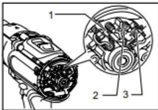
1. Arm 2. Spring 3. Recessed part
