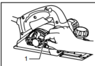
1. Carbon brushes
