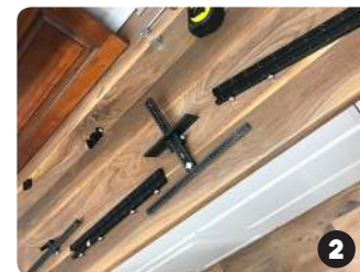
Use TP-1934 with long hardware/shelf pin extension and the TP-ERA
