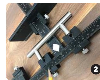
slide two drill bushings onto the tp-1934 Using the same measurements
