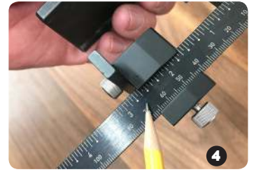
Match the sliding end stop with your bottom measurement and tighten
