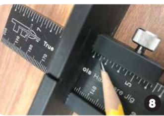
Set the Large Stop and tighten at desired location
